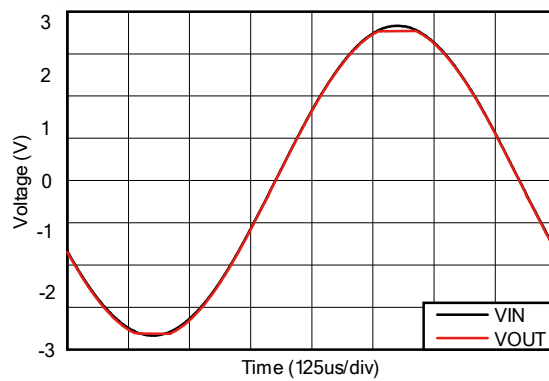
Figure 14. Output Waveform Devoid of Phase Reversal During an Input Overdrive Condition
