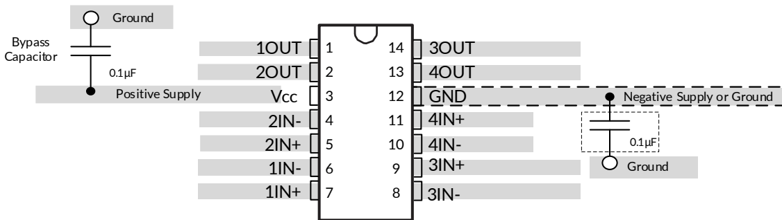
Figure 9. LM2901 Layout Example
