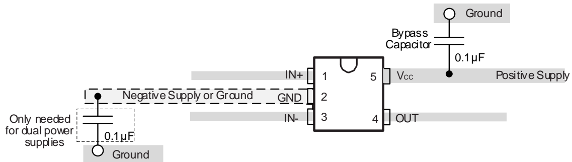
Figure 39. RS331-Q1 Layout Example
