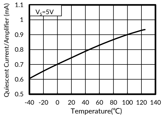
Figure 6. Quiescent Current vs Temperature
