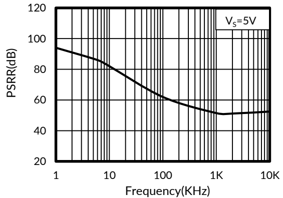
Figure 4. Power-Supply Rejection Ratio vs Frequency
