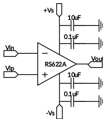
Figure 15. Amplifier with Bypass Capacitors
