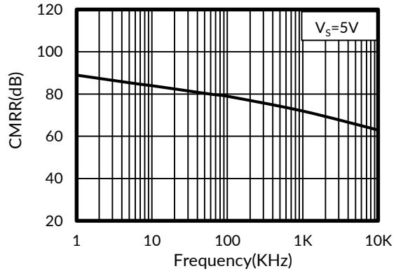
Figure 2. Common-Mode Rejection Ratio vs Frequency
