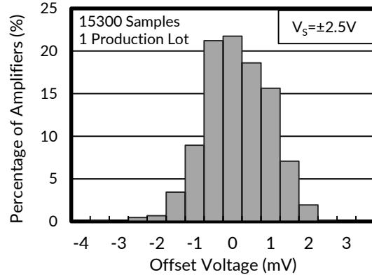
Figure 14. Offset Voltage Production Distribution
