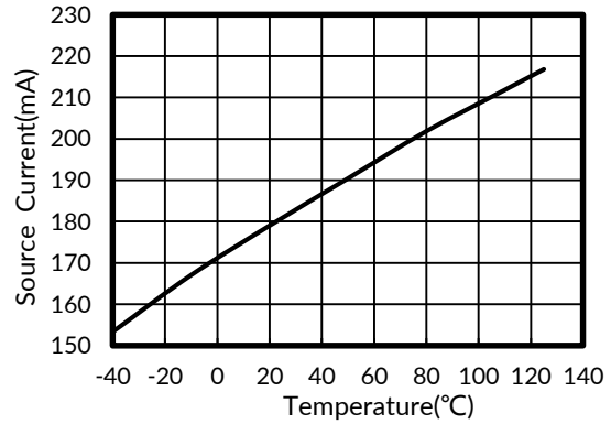
Figure 8. Source Current vs Temperature
