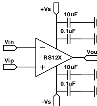
Figure 10. Amplifier with Bypass Capacitors
