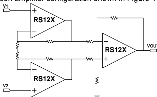
Figure 11. Amplifier instrumentation amplifier
