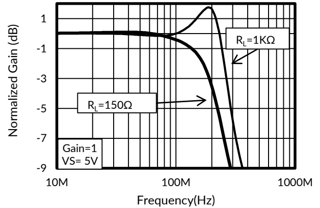
Figure 2. -3dB_GW
