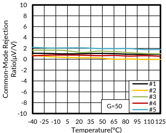
Figure 5. Common-Mode Rejection Ratio vs Temperature
