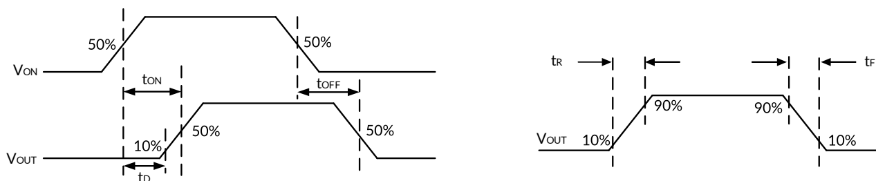
Figure 2. Switch Turn-On and Turn-Off Delay Times
