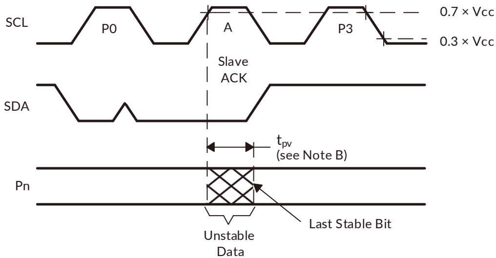
Write Mode ( R/\bar{W} = 0 )
