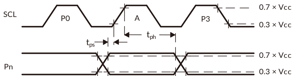
Read Mode ( R/\bar{W} = 1 )
