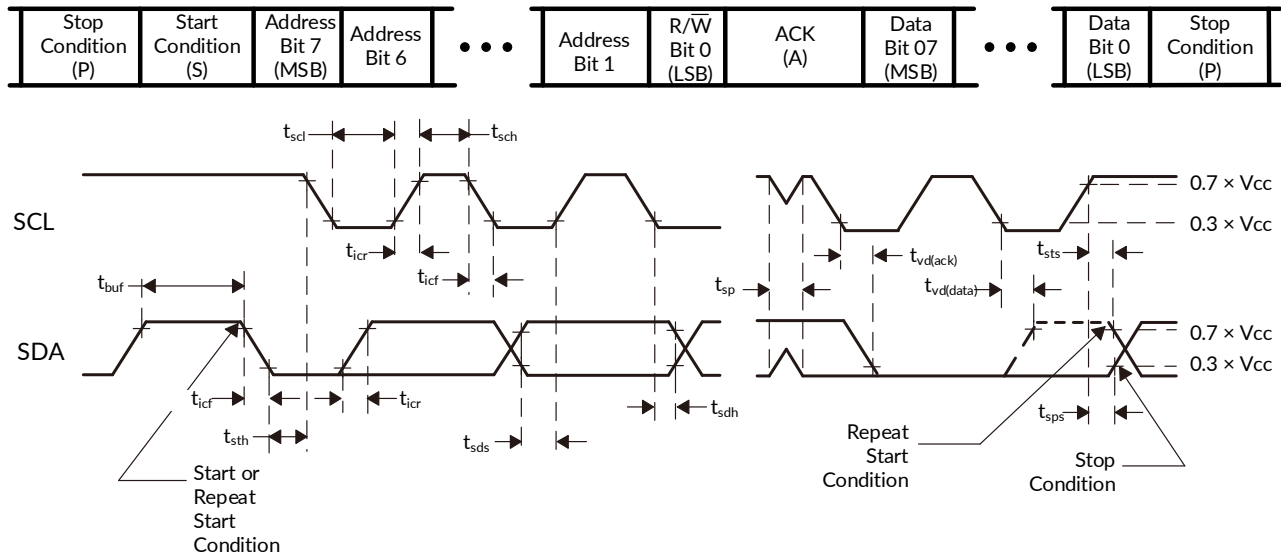
VOLTAGE WAVEFORMS
