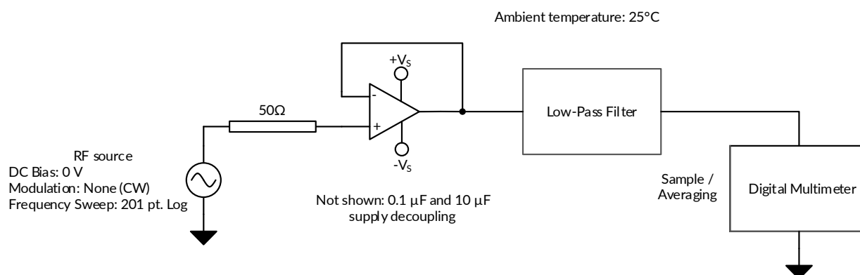
Figure 17. EMIRR IN+ Test Configuration Schematic
