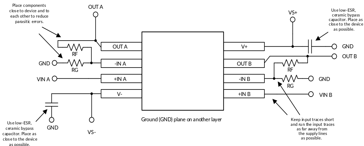
Figure 21. Layout Example
