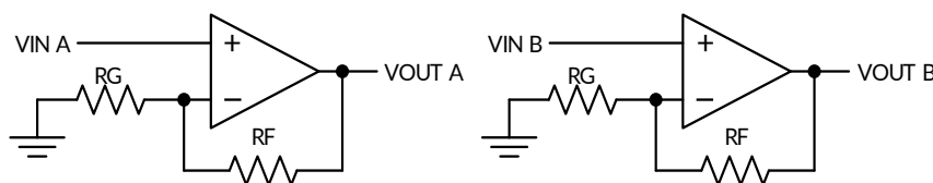
Figure 20. Schematic Representation
