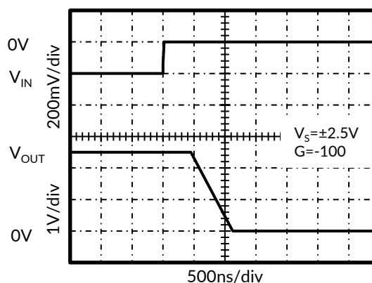
Figure 12. Positive Overload Recovery
